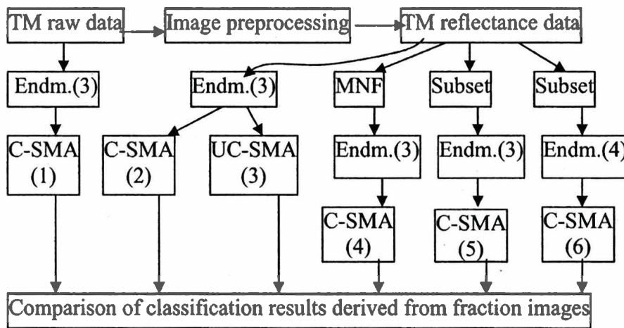
Figure 3. Different image-processing methods for LULC classification. (1) Raw-c (C-SMA 1 ): using constrained solution in SMA with three endmembers (i.e. shade, green vegetation and soil) on raw six-band Landsat TM data; (2) Ref-c (C-SMA 2 ): using constrained solution in SMA with three endmembers on six-band Landsat TM reflectance image; (3) Ref-uc (UC-SMA 3 ): using unconstrained solution in SMA with three endmembers on six-band Landsat TM reflectance image; (4) MNF-c (C-SMA 4 ): using constrained solution in SMA with three endmembers on the first four MNF components; (5) Subset-c (C-SMA 5 ): using constrained solution in SMA with three endmembers on bands Landsat TM 3, 4, 5, and 7; and (6) Subset-4c (C-SMA 6 ): using constrained SMA with four endmembers (i.e. green vegetation, shade, bright soil and dark soil) on bands TM 3, 4, 5, and 7.
